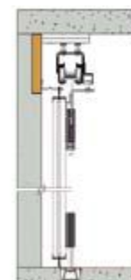
Posa soffitto in luce Installation in the opening Einbau in der Öffnung
